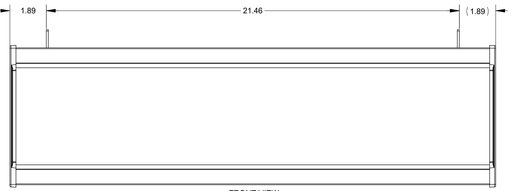
FRONT VIEW ALPHA 4080 MNS BACK-TO-BACK UNITS (APPROXIMATE HANGING WEIGHT = 16 LBS)
