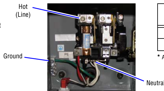
Disconnect box - inside view
